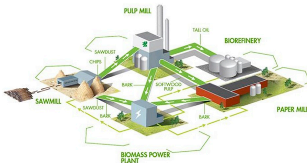
Fig. 6. UPM kaukas mill (lapeenranta, Finland). Source: Biofore [25].
